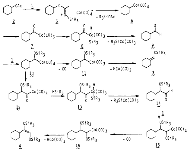
Scheme I. Proposed Mechanism of the Catalytic Reaction
